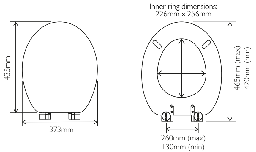
General seat dimensions
