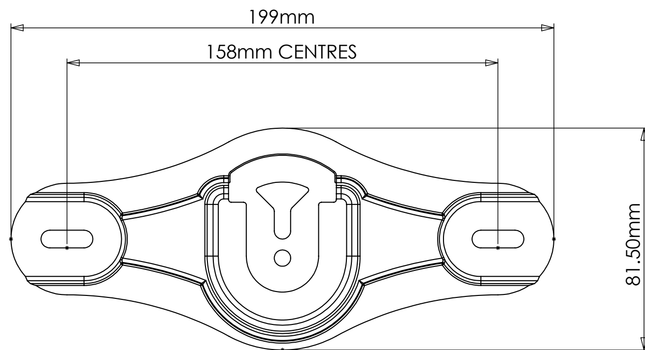
WALL BRACKET
