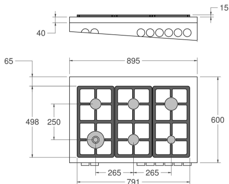
WORKTOP DETAILS
