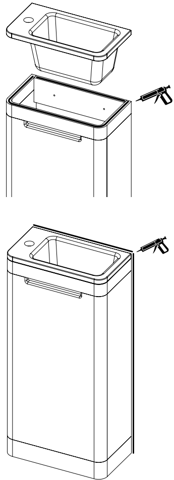
Fig. 2 Silicone Placement
