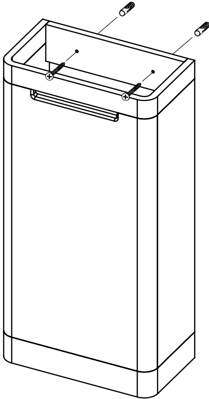
Fig. 1 Fixing Holes
