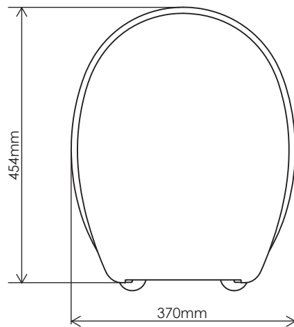
General seat dimensions
